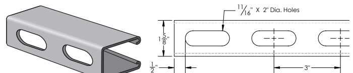
ELEMENTS OF SECTION – PS 150 2T3
