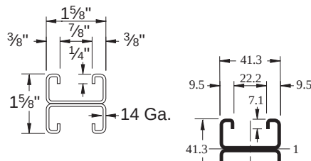
ELEMENTS OF SECTION – PS 500 2T3
