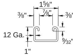
ELEMENTS OF SECTION – PS 400
