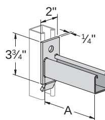
(PS 808 T1 - Slot Up)
