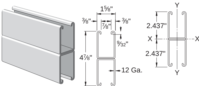
ELEMENTS OF SECTION – PS 150 2T3
