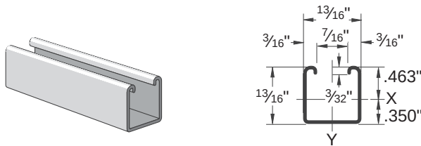
BEAM LOADING – PS 600J
