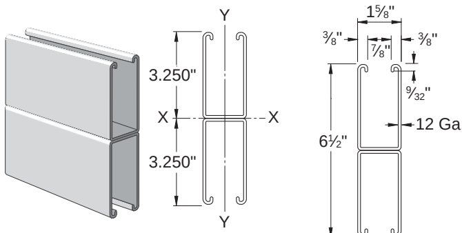
ELEMENTS OF SECTION – PS 100 2T3
