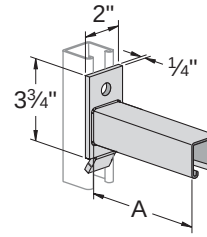
(PS 808 T2 - Slot Down)
