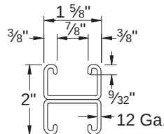
ELEMENTS OF SECTION – PS 400 2T3
