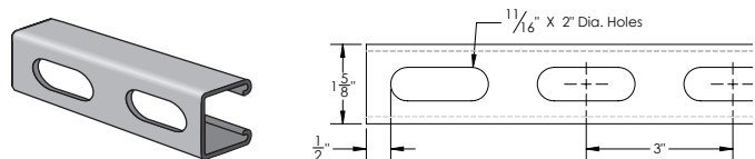
ELEMENTS OF SECTION – PS 200 2T3
