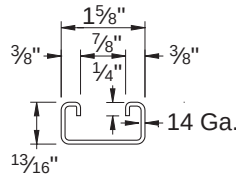
ELEMENTS OF SECTION – PS 500
