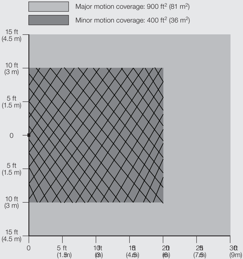
NEMA WD7 Test Grid Coverage (High Sensitivity Setting)
